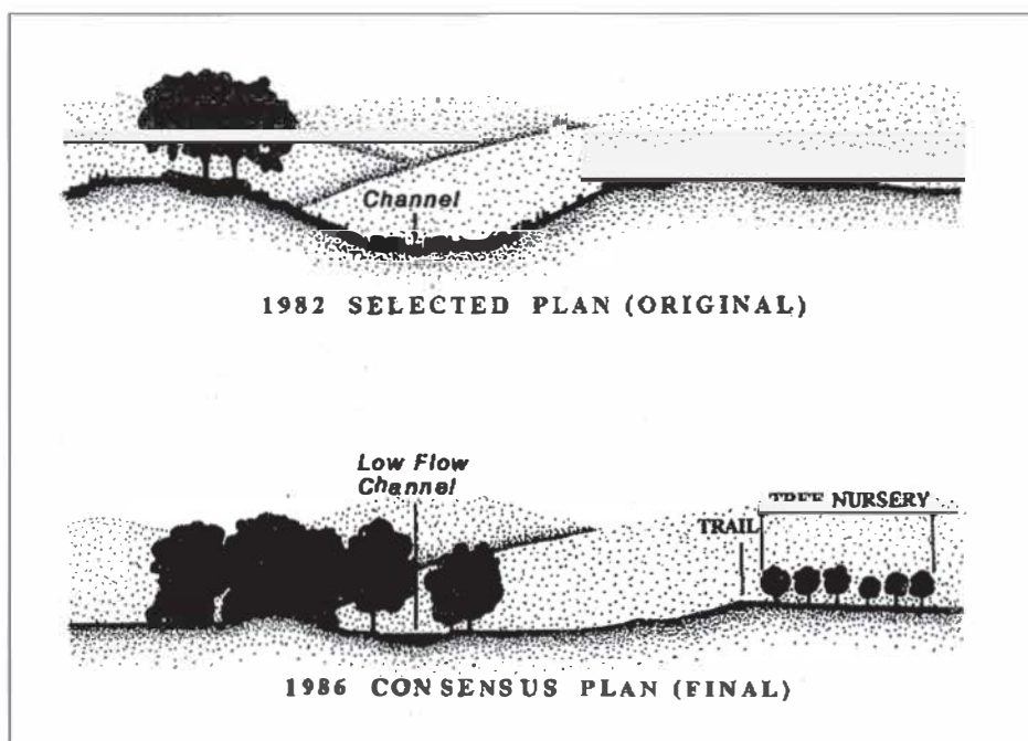
Figure 20 - These crosssections illustrate the two alternative creek channel designs for Wildcat and San Pablo Creeks. The original 1982 plan utilizes a typical box cross-section, high-capacity channel with little or no adjacent floodplain; the 1986 plan eventually implemented includes a shallow low flow channel with floodplain intact allowing trails, tree nursery, etc.
